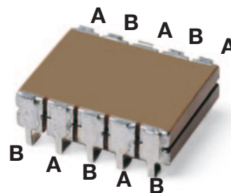
Interdigitated configuration results in reduced ESL
