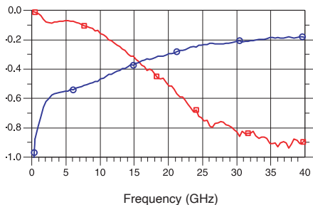
Transmission and Return Loss (S21, S11)
