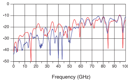
Return Loss (S11)
