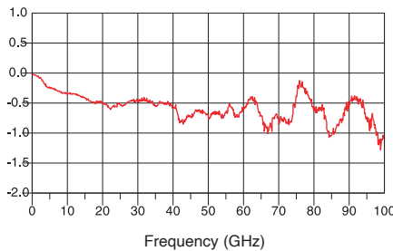
Transmission Loss (S21)
