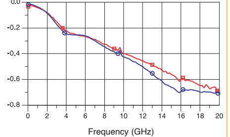
Transmission Loss over Temperature (S21)
