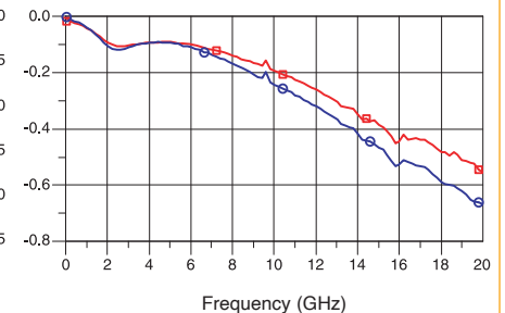
Transmission Loss over Temperature (S21)
