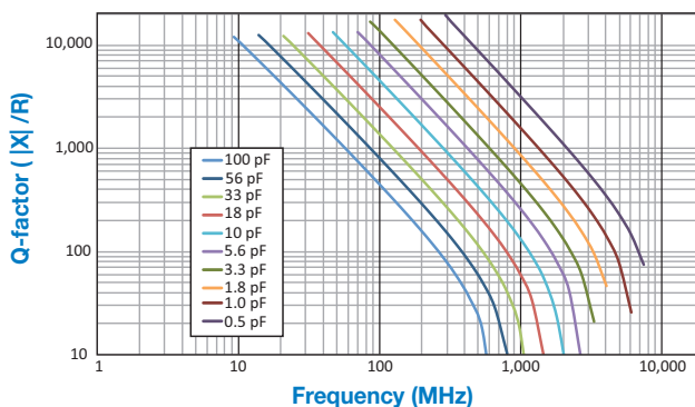
0603NPO Q vs. FREQUENCY
