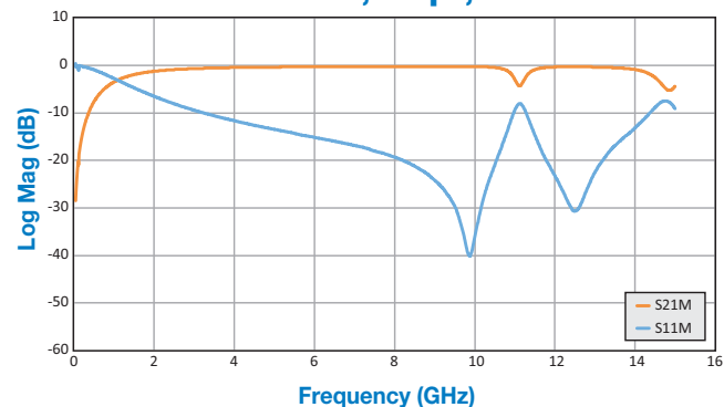
0603NPO, 1.5pF, S2P
