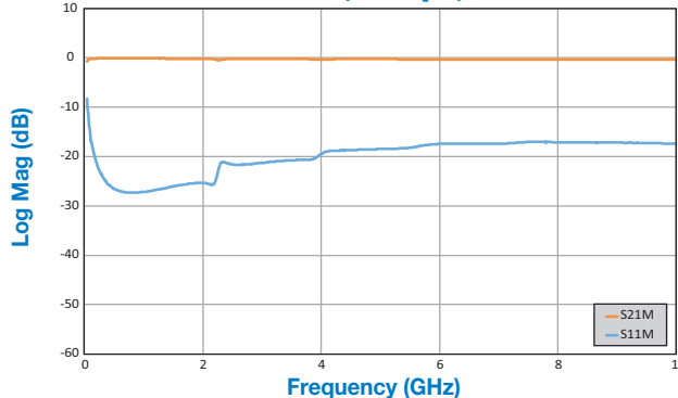
0603NPO, 100pF, S2P
