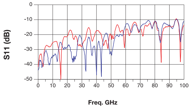
Return Loss (S11)
