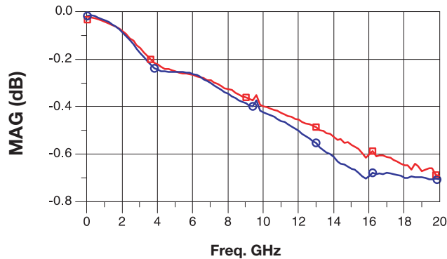
Transmission Loss Over Temperature (S21)
