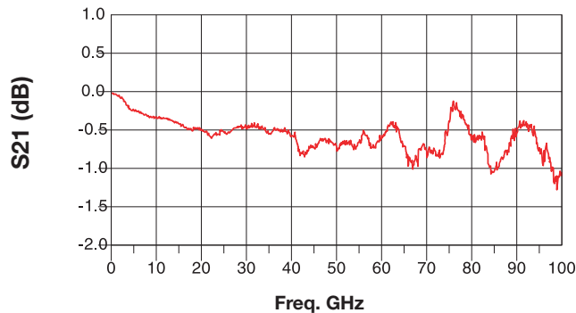
Transmission and Return Loss (S21)
